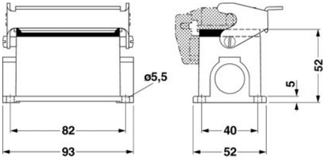
Dimensioned drawing
